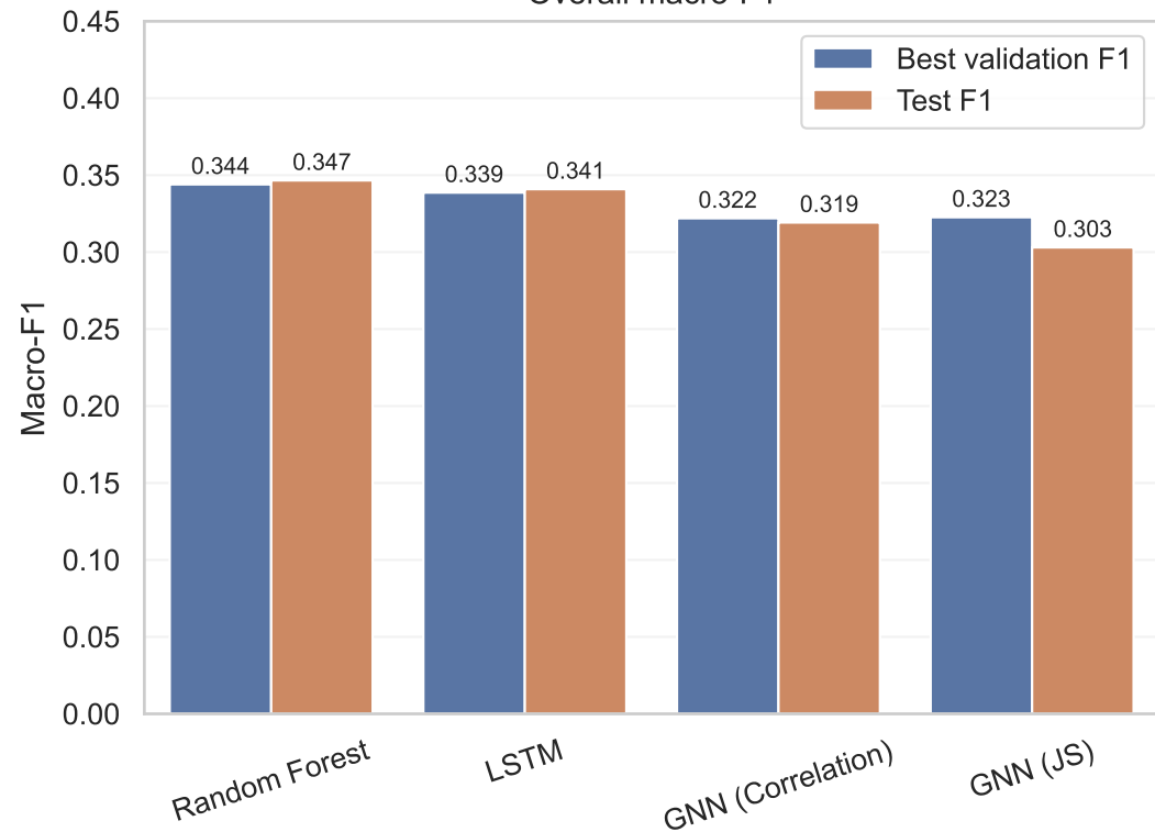
Overall macro-F1
